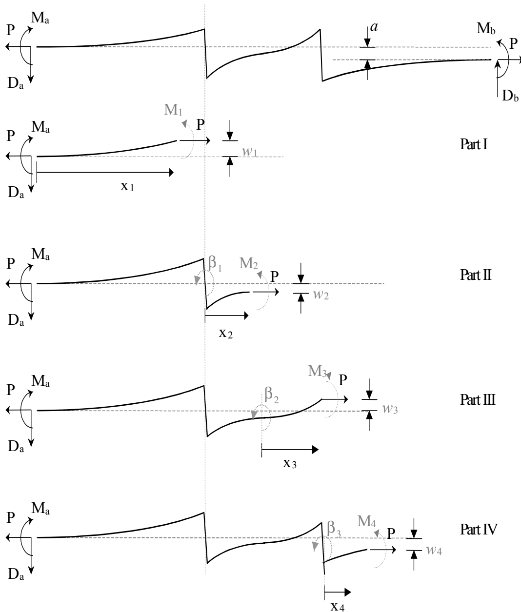
Figure 2 Deflection of neutral line for a three-rievet lap-splice joint.
