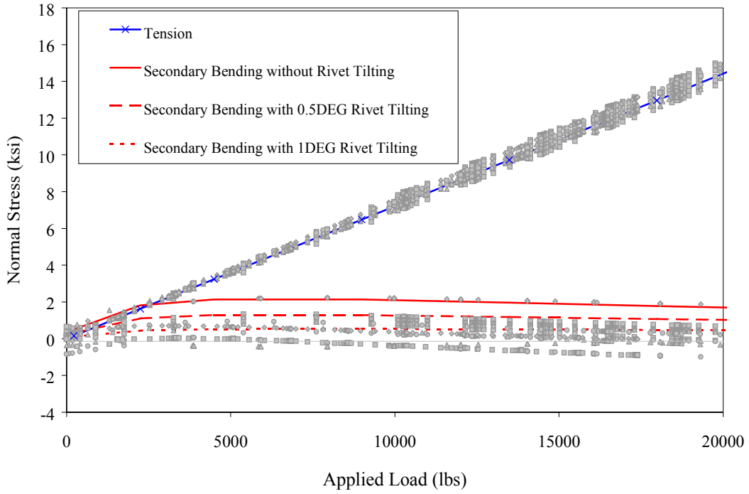
Figure 6 JOINT I: lap-splice joint Secondary bending and Tension stresses
