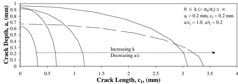
Figure 8 Crack Shape Development as a Function of the Bending Factor, k
