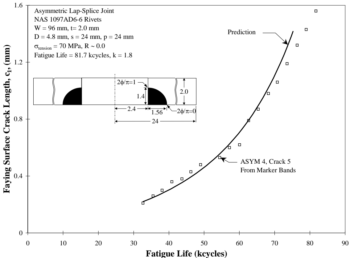
Figure 22 Crack Growth Prediction for Asymmetric Lap Splice Joint, Part Through Crack
