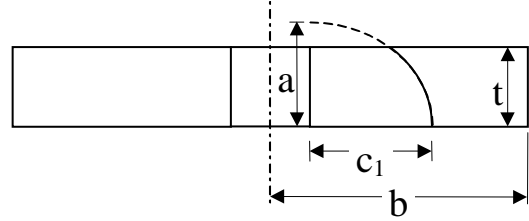
Figure 1 Part-Elliptical Through Crack Geometry
