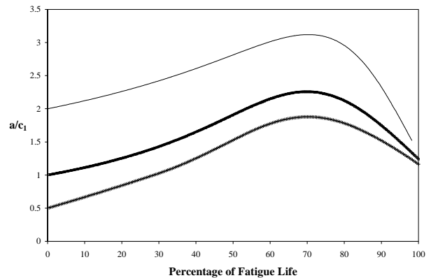
Figure 7 Crack Shape Development during the Fatigue Life
