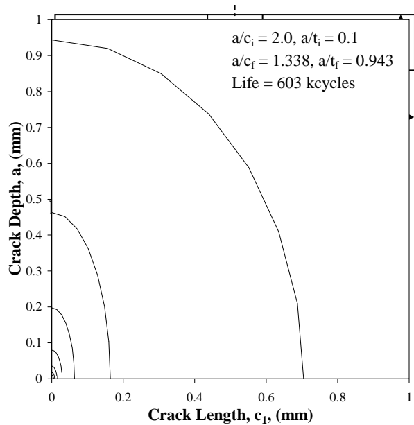
Figure 6 Crack Shape Development with Initial a/c_1 = 2.0
