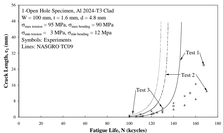
Figure 13 TC09 Verification Remote Tension and Secondary Bending
