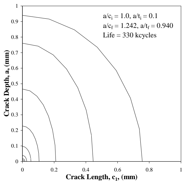
Figure 5 Crack Shape Development with Initial a/c_1 = 1.0
